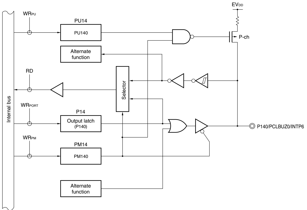
Figure 4-27. Block Diagram of P140
