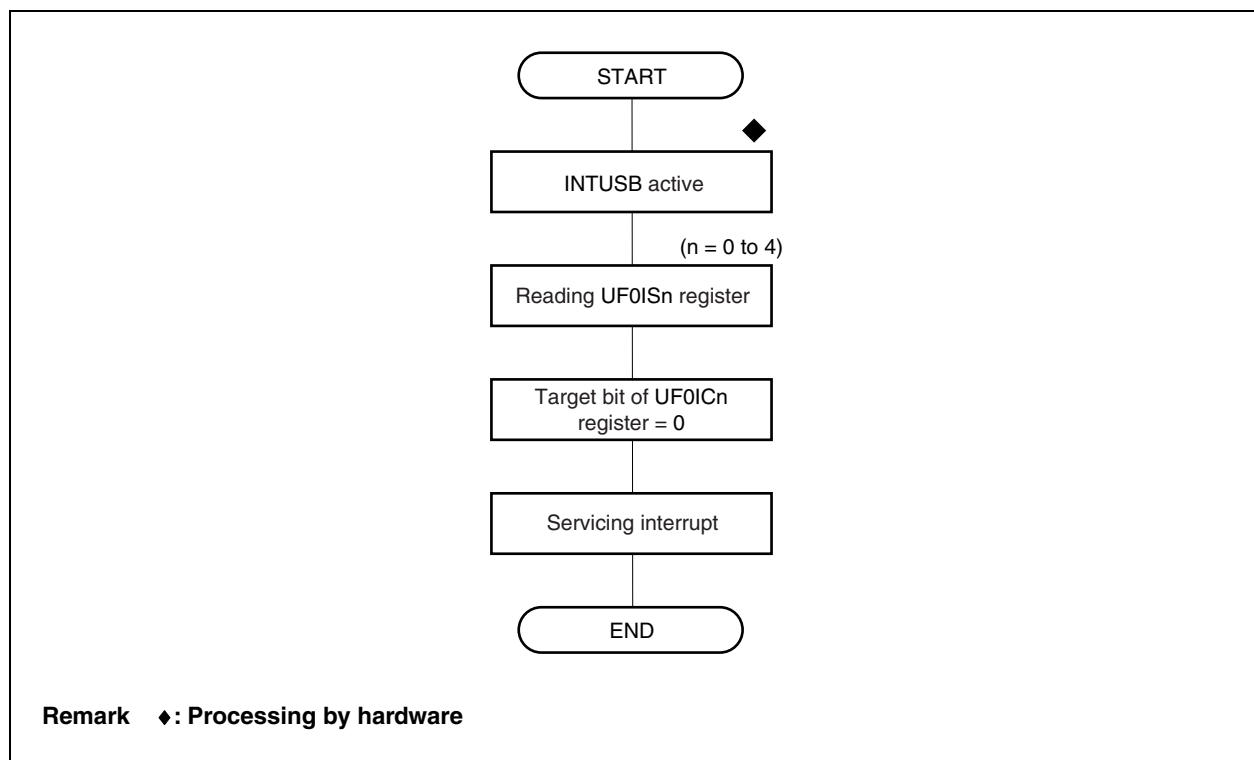
Figure 13-17. Interrupt Servicing
