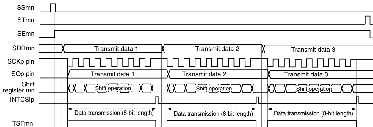
Figure 11-29. Timing Chart of Master Transmission (in Single-Transmission Mode) (Type 1: DAPmn = 0, CKPmn = 0)
