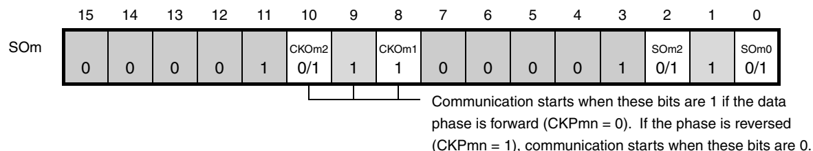
Figure 11-25. Example of Contents of Registers for Master Transmission of 3-Wire Serial I/O (CSI00, CSI10, CSI20)
