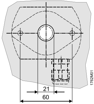
Drilling plan
