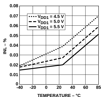
Figure 4. INL (%) vs. Temperature.
