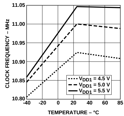
Figure 17. Clock Frequency vs. Temperature.
