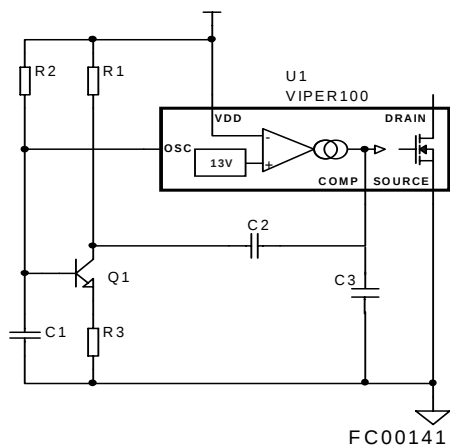
Figure 20. Slope Compensation
