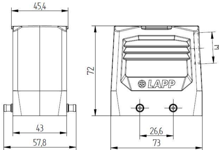
Side cable entry
