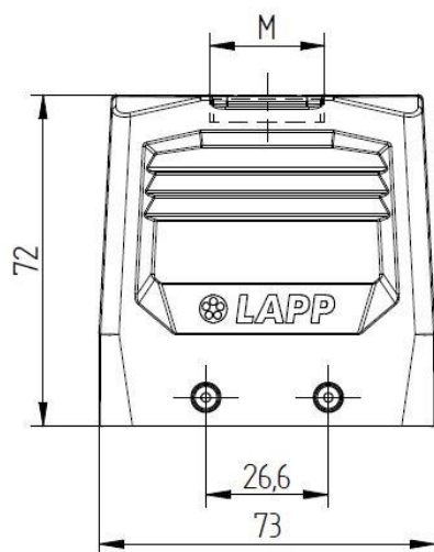
Top cable entry
