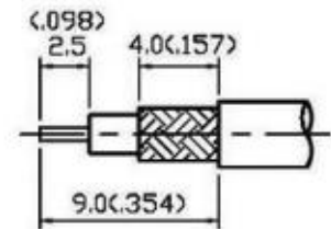
STRIPPING DIMENSION
