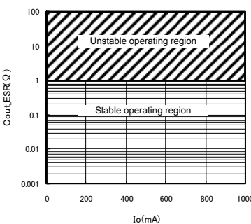
C out_ESR vs I o 1.0V ≤ V O < 3.0V (Reference data)
