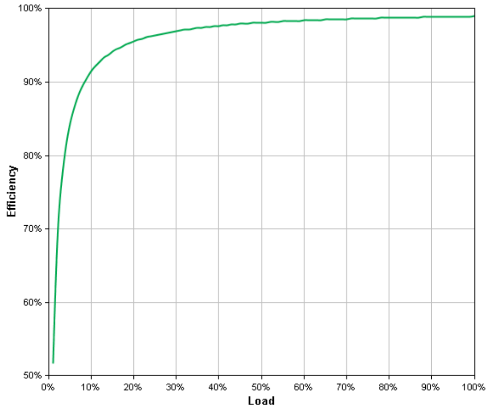
APC Back-UPS 500, 230V (BK500EI)
