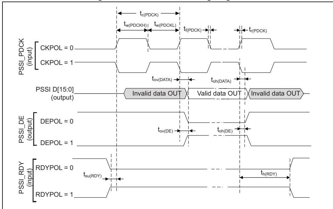
Figure 57. PSSI transmit timing diagram
