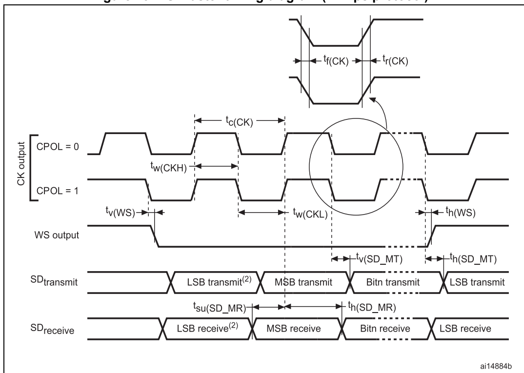
Figure 75. I 2 S master timing diagram (Philips protocol) (1)
