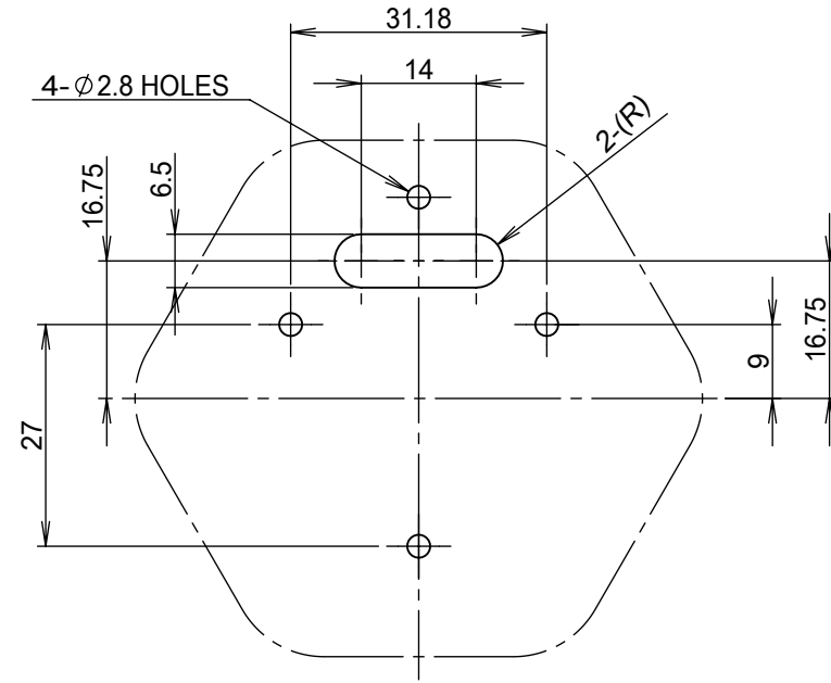
Machining dimensions for sheet metal mounting holes (References)
