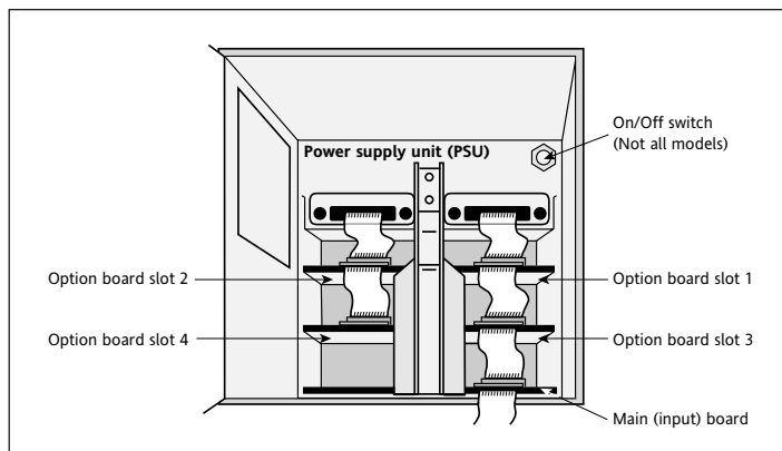
Exploded view
