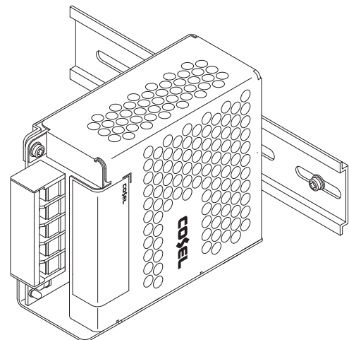
Fig.5.18 Power supply installed on a DIN rail (PLA50F)
