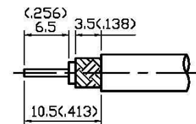
STRIPPING DIMENSION
