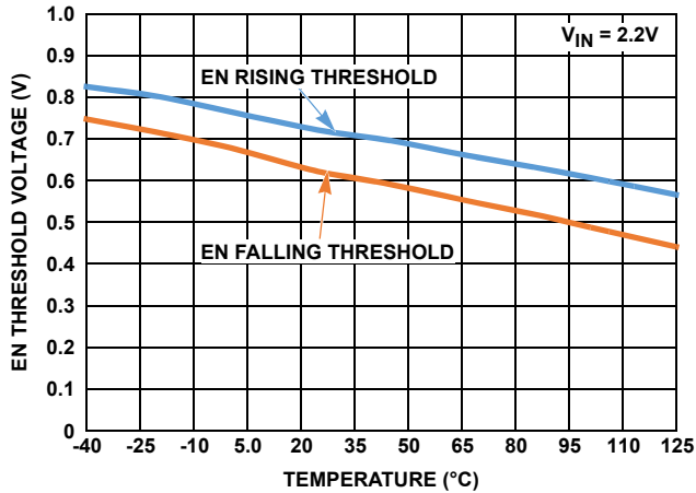
FIGURE 12. EN THRESHOLDS vs TEMPERATURE
