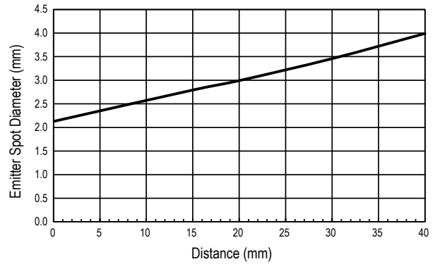
Typical Emitter Spot Diameter vs. Distance
