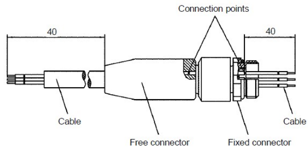
Fig.4 Contact resistance arrangement
