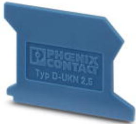
End cover, Length: 43.5 mm, Width: 1.5 mm, Height: 42 mm, Color: blue
