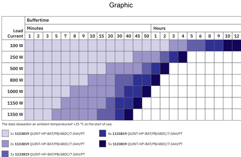
QUINT HP UPS 1.5 kVA buffer times
