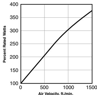
Fig. 14: Percent of Free Air Rating for Typical Resistor Cooled by Forced Air Circulation.
