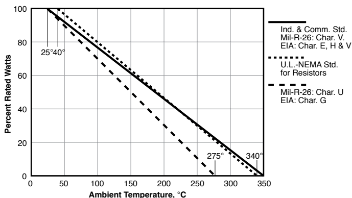
Fig. 3: Derating for ambient temperature.
