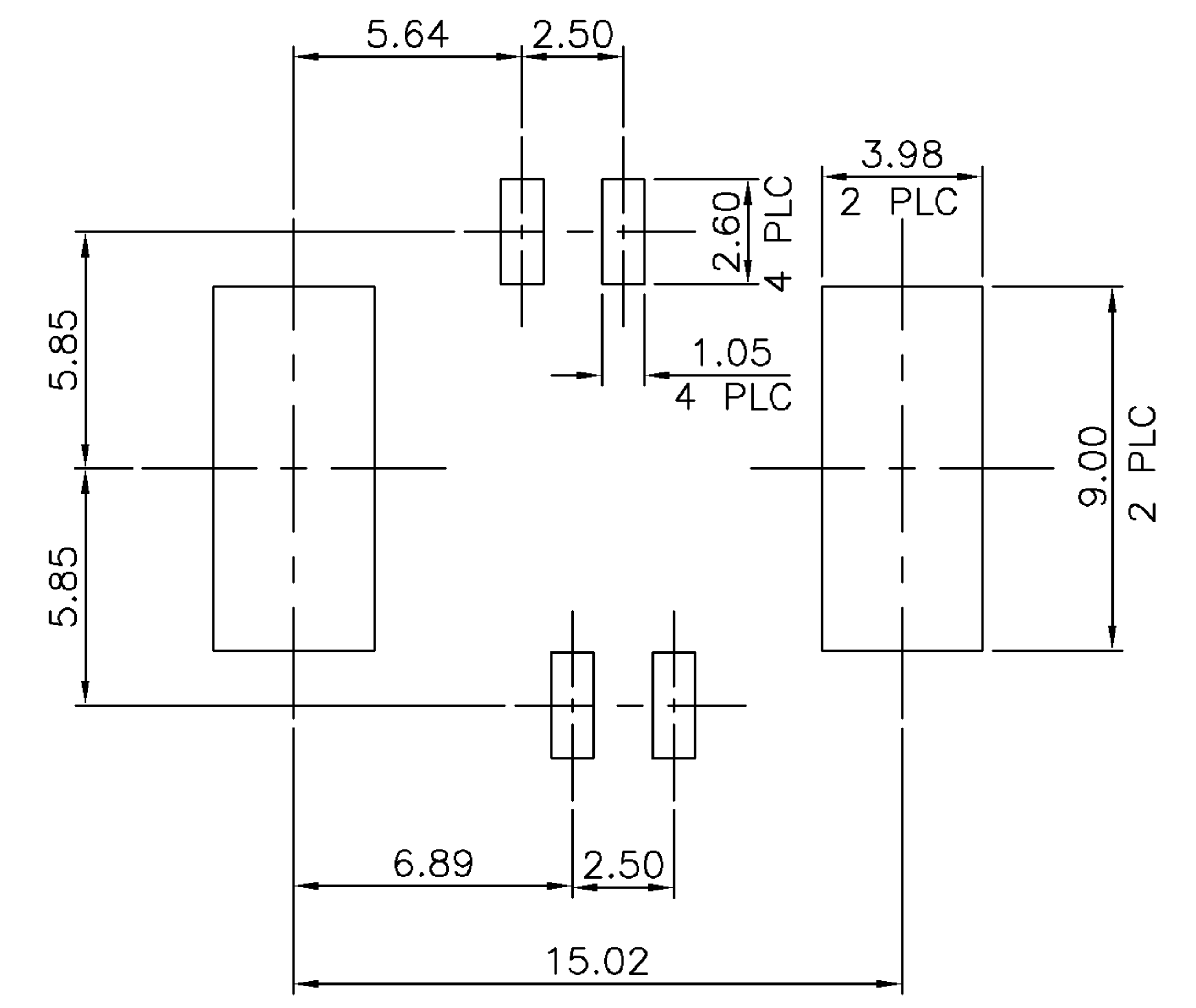
RECOMMENDED PCB LAYOUT (TOLERANCE: ±0.05)
