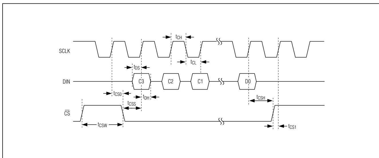
Figure 1. Timing Diagram
