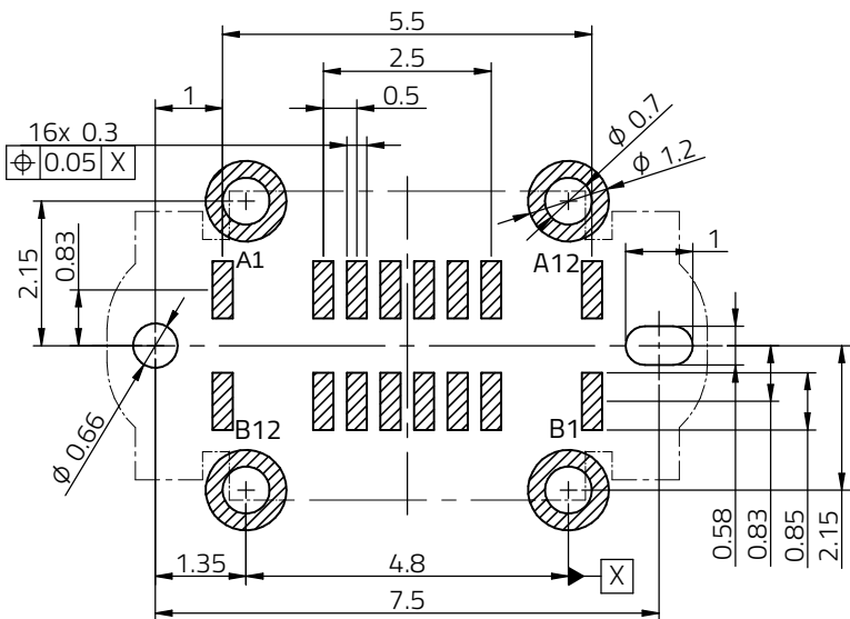
General tolerance ±0.05
