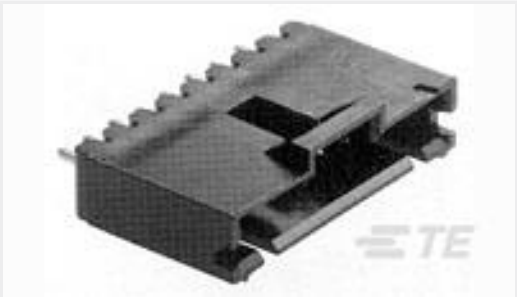
TE Part #5-104363-7 08 MTE HDR SRST LATCH .100CL
