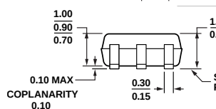
Figure 35. 5-Lead Thin Shrink Small Outline Transistor Package [SC70] (KS-5) Dimensions shown in millimeters
