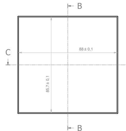
Body enclosure
