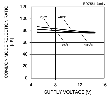
Fig. 18 Common Mode Rejection Ratio – Supply Voltage ( V_{DD}=12[V] )
