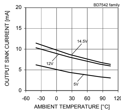
Fig. 81 Output Sink Current - Ambient Temperature ( V_{OUT}=V_{DD}-11.6[V] )
