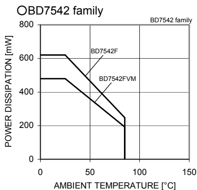
Fig. 70 Derating Curve
