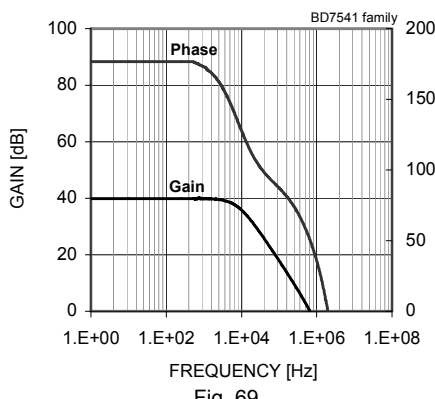
Gain - Frequency
