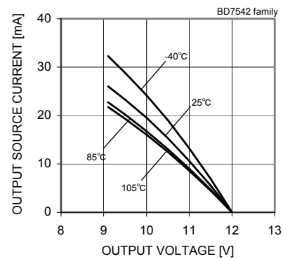
Fig. 78 Output Source Current - Output Voltage ( V_{DD}=12[V] )
