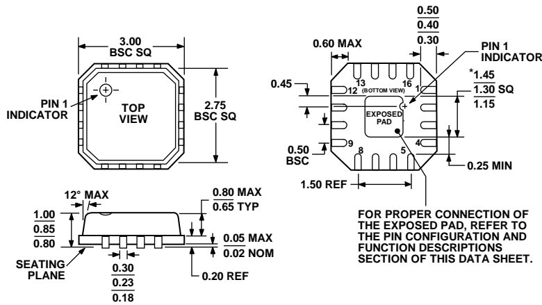
Figure 77. 16-Lead Lead Frame Chip Scale Package [LFCSP_VQ] 3 mm x 3 mm Body, Very Thin Quad (CP-16-2) Dimensions shown in millimeters
