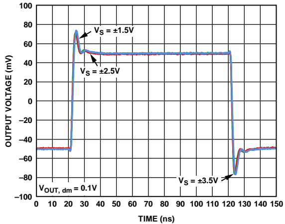
Figure 50. Small Signal Transient Response for Various Supplies (LFCS)
