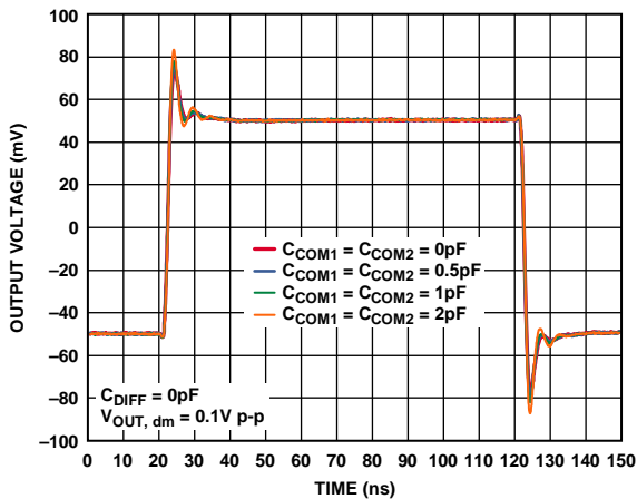
Figure 51. Small Signal Transient Response for Various Capacitive Loads (LFCS)
