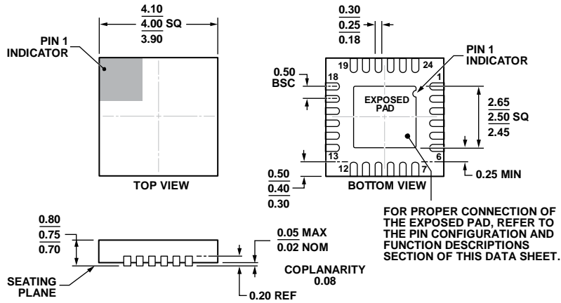
Figure 79. 24-Lead Lead Frame Chip Scale Package [LFCSP_WQ] 4 mm × 4 mm Body, Very Very Thin Quad (CP-24-7) Dimensions shown in millimeters
