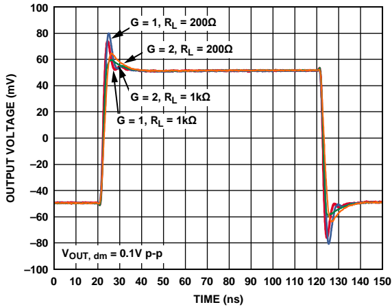
Figure 49. Small Signal Transient Response for Various Gains and Loads (LFCS)
