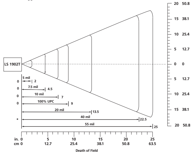
LS 1902T Triggered Bar Code Decode Zone
