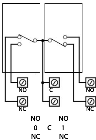
Terminals 0 and 1
