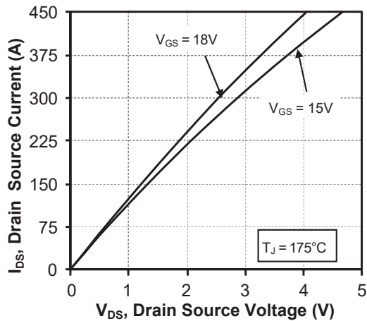
Figure 1-3. Output Characteristics, T_J = 175^\circ\text{C}
