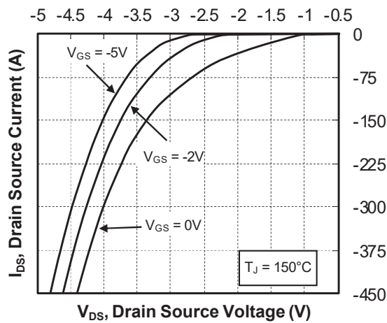
Figure 1-11. Body Diode Characteristics, T_J = 150^\circ\text{C}
