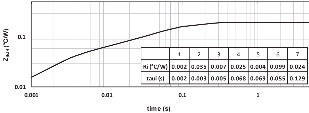
Figure 1-6. Junction-to-Heatsink Thermal Impedance
