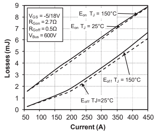
Figure 1-4. Switching Energy vs. Current
