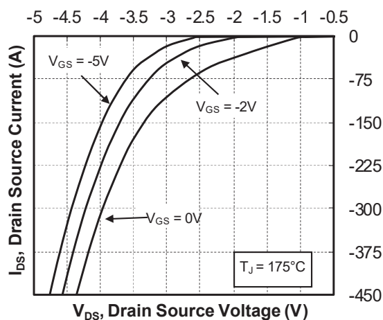
Figure 1-13. Body Diode Characteristics, T_J = 175^\circ\text{C}
