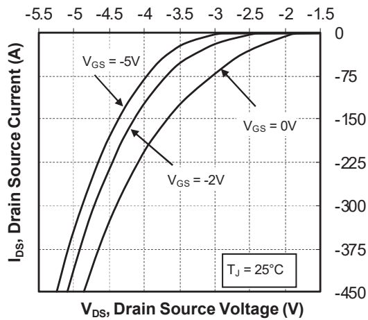
Figure 1-9. Body Diode Characteristics, T_J = 25^\circ\text{C}
