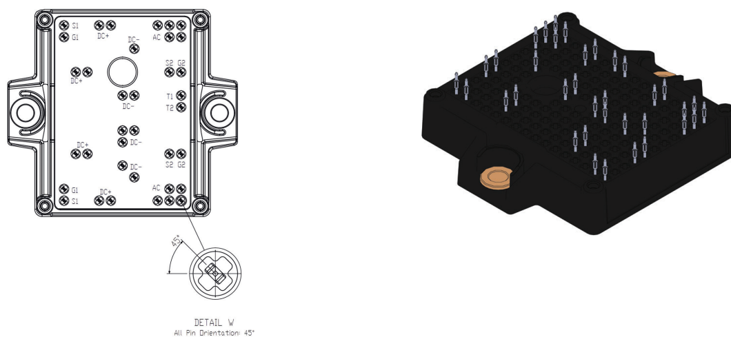
Figure 2. Pinout Location
