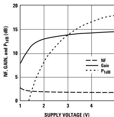
Figure 3. Gain, NF and P1dB vs. supply voltage at 1900 MHz.
