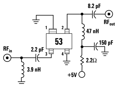
Figure 21. Schematic for 1900 MHz LNA design.
