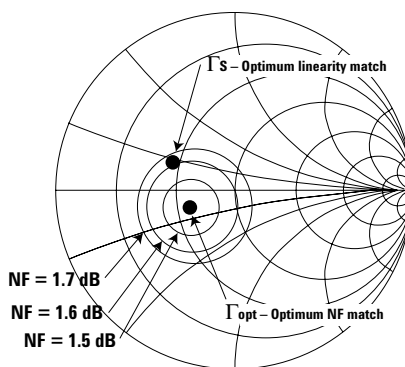
Figure 8. Noise figure performance.
