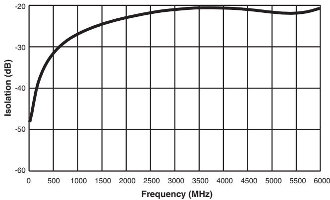
Isolation Across Contacts (RF Note 4)
