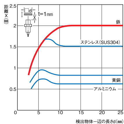
形E2E2-X5MC□/-X5MY□
