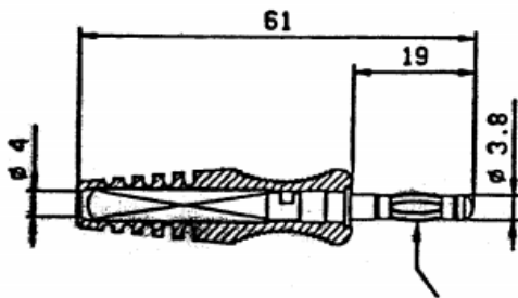
Cage spring for socket dia 4.0mm
