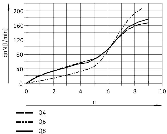
Standard nominal flow rate q_{nN} at 0.6 \rightarrow 0.5 MPa as a function of spindle revolutions n for threaded connection G1/8, R1/8 (supply air)
