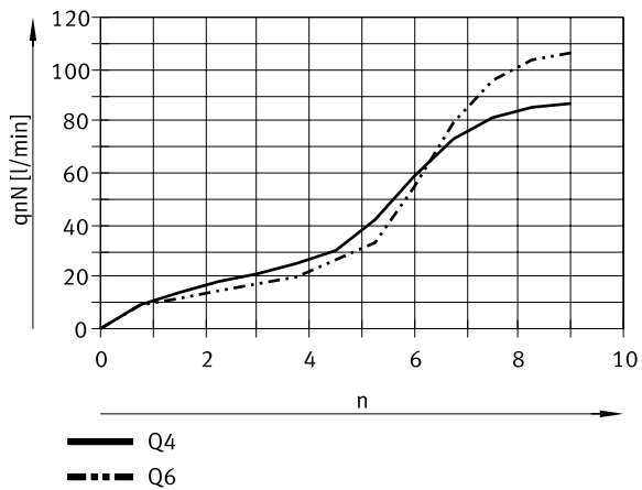
Standard nominal flow rate q_{nN} at 0.6 \rightarrow 0.5 MPa as a function of spindle revolutions n for threaded connection M5, M7 (supply air)
