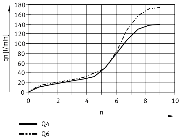
Standard flow q_n at 0.6 \rightarrow 0 MPa as a function of spindle revolutions n for threaded connection M5, M7 (supply air)
