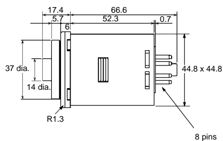
Dimensions with Back Connecting Socket P3G-08/P3GA-11
