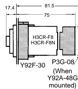
Dimensions with Back Connecting Socket P3G-08/P3GA-11
