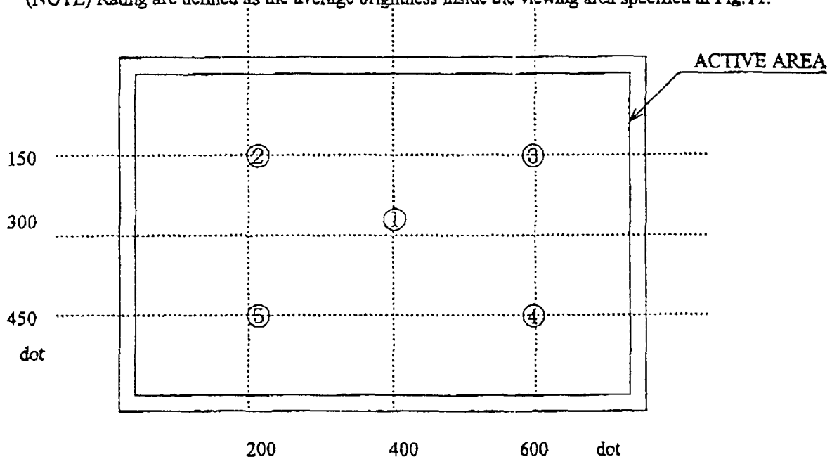
Fig.11 Measuring points (1-5)
