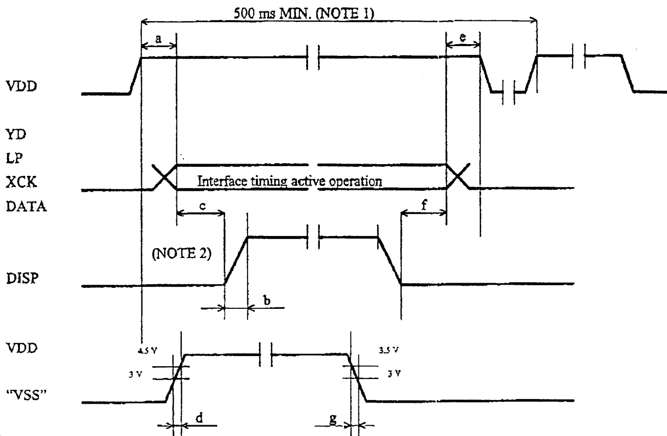
Fig. 12 Supply voltage sequence condition
