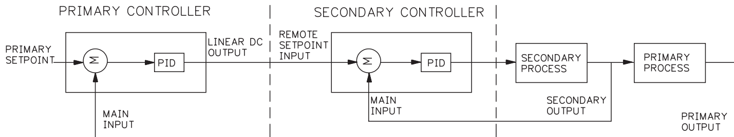
Figure 35, Cascade Control
