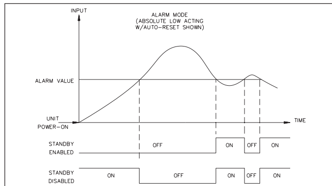
Figure 18, Alarm Standby Delay Sequence
