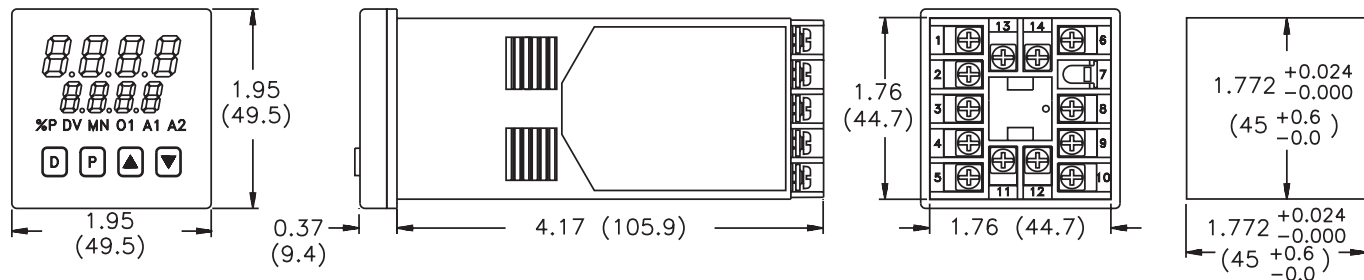
Figure 43, Dimensions
