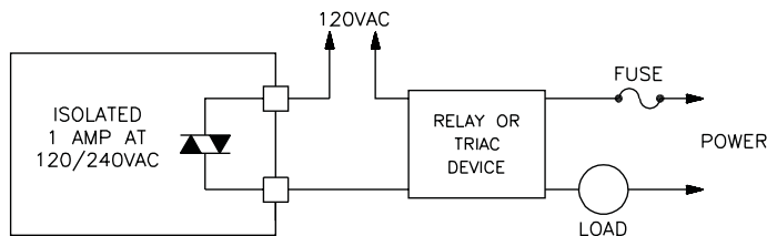
Figure 9, Triac Output
