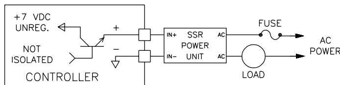
Figure 8, Logic/SSR Output
