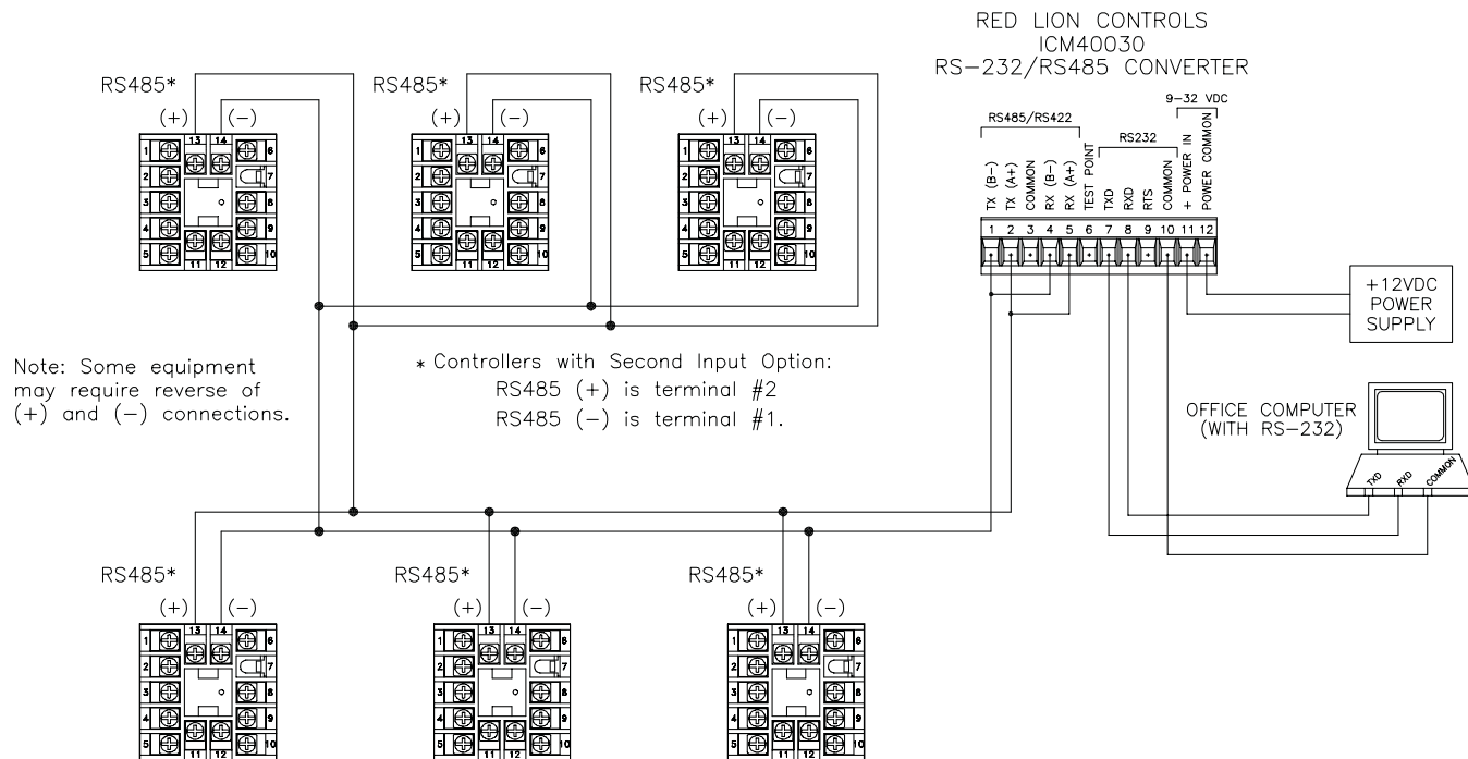
Figure 10, Connecting to a Host Terminal
