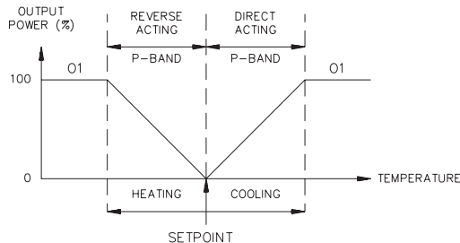
Figure 30, Proportional Band
