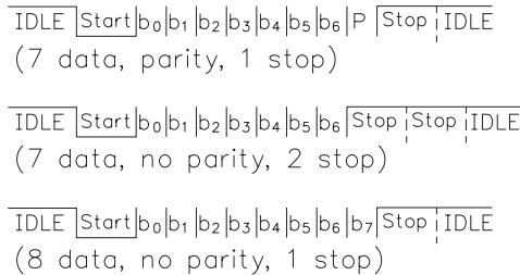
Figure 36, Character Frame
