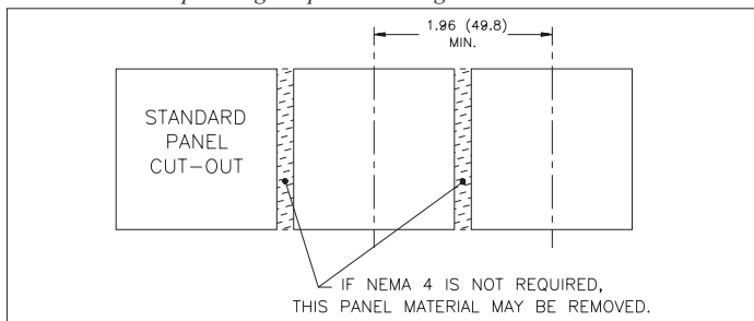
Figure 3, Multiple Unit Stacking Horizontal Arrangement
