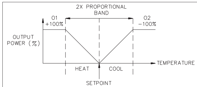
Figure 19, Heat/Cool Operation (db=0)
