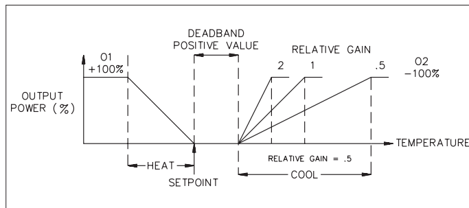
Figure 20, Heat/Cool Operation (db>0)
