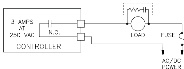
Figure 7, Relay Output
