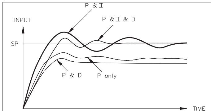
Figure 33, Typical Response Curve
