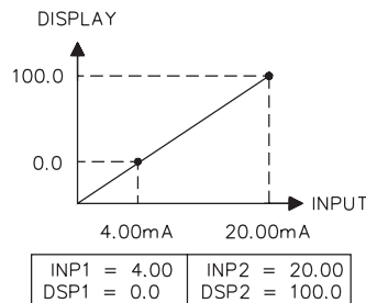
Figure 14, Scaling Points
