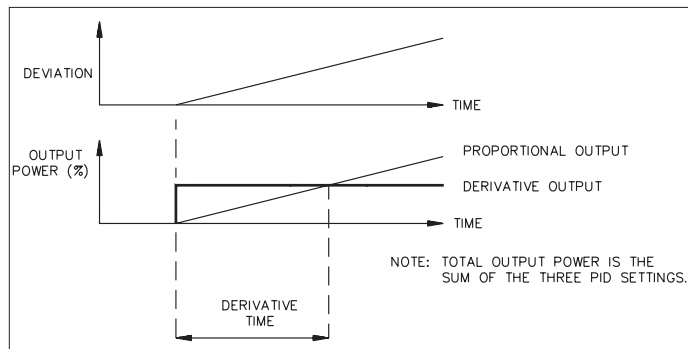
Figure 32, Derivative Time
