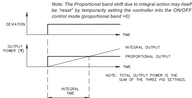
Figure 31, Integral Time
