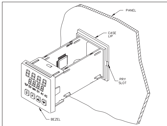
Figure 2, Bezel Assembly
