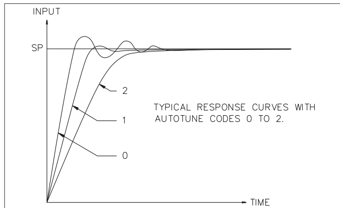
Figure 28, Auto-Tune Code
