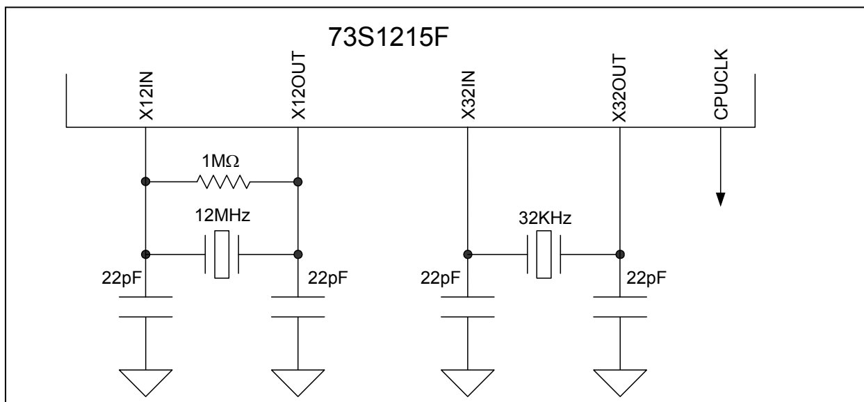
Figure 4: Oscillator Circuit
