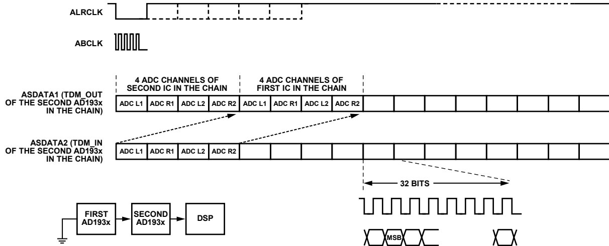
Figure 22. ADC TDM Daisy-Chain Mode (512 f_s BCLK, Two-AD1938 Daisy Chain)
