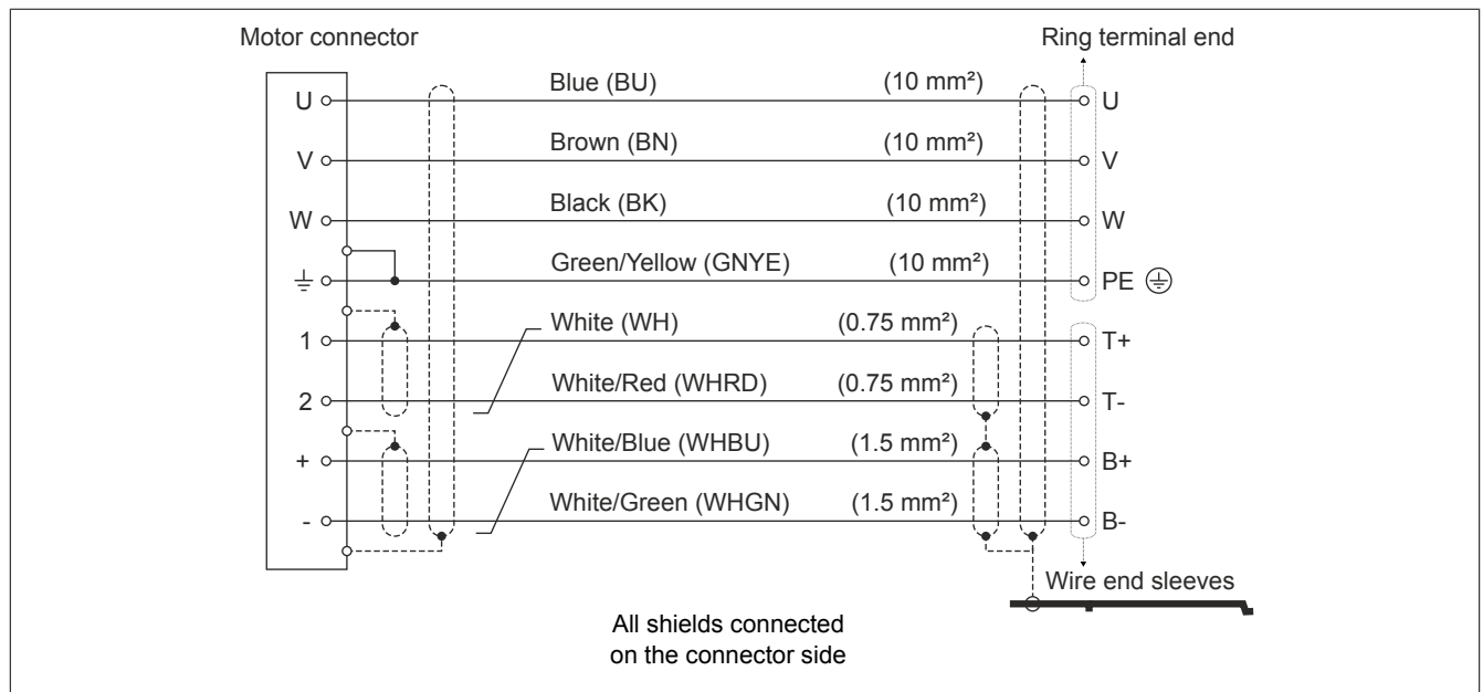
Figure 1: 8BCMxxxx.1525B-0 motor cables - Cable diagram
