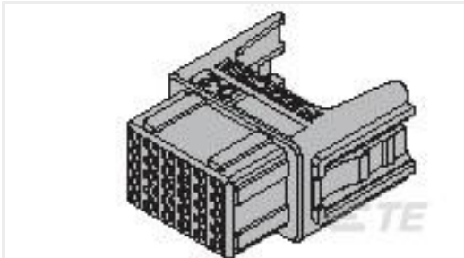
TE Part #1871416-1 DYNAMIC D-4800 REC HSG 8P WITH HTS CONN
