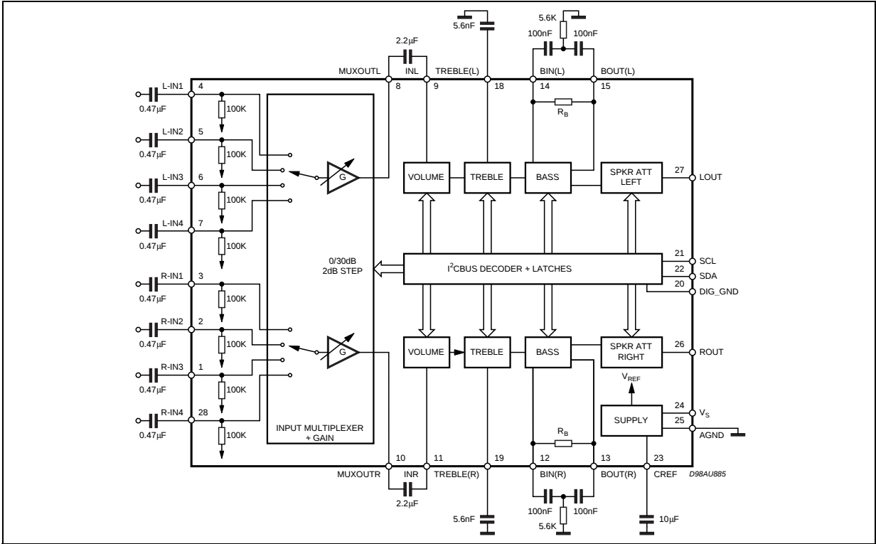
Figure 4. Test Circuit
