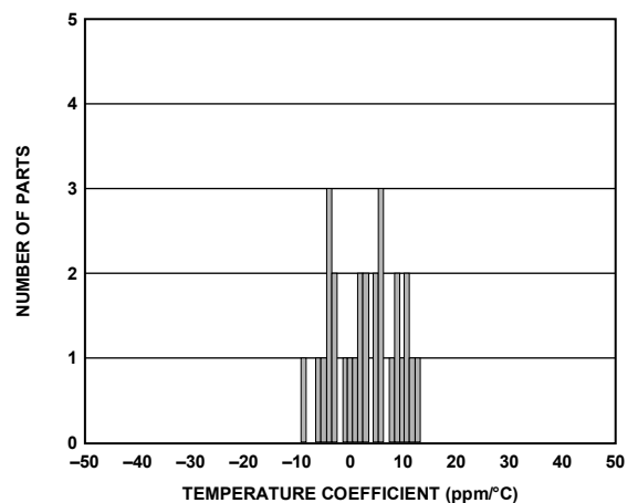
Figure 7. ADR125 Temperature Coefficient
