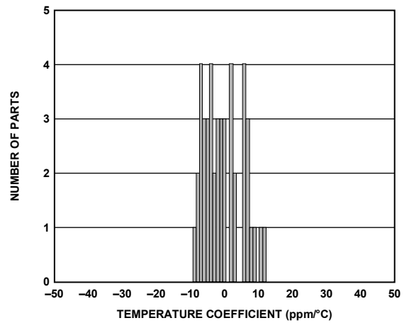
Figure 6. ADR121 Temperature Coefficient
