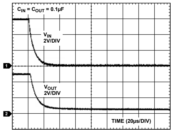
Figure 37. ADR125 Turn-Off Response
