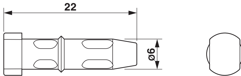
Dimensional drawing
