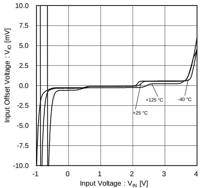
Figure 18. Input Offset Voltage vs Input Voltage ( V_{DD}=3.0\text{ V} )
