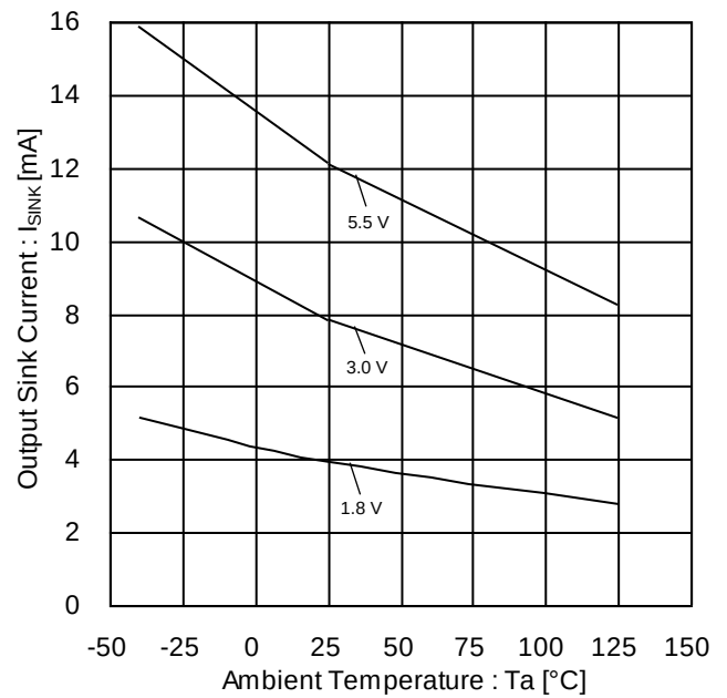
Figure 10. Output Sink Current vs Ambient Temperature ( V_{OUT}=V_{SS}+0.4 V)
