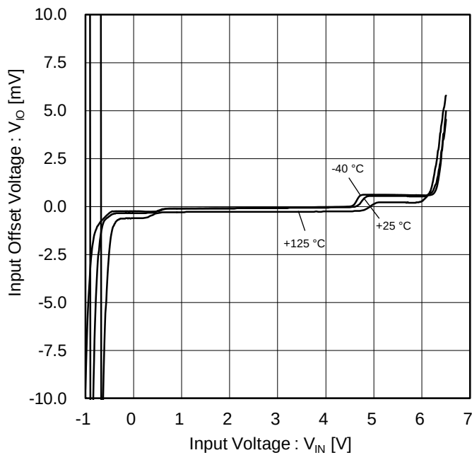
Figure 19. Input Offset Voltage vs Input Voltage ( V_{DD}=5.5\text{ V} )
