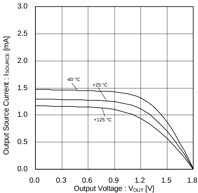
Figure 11. Output Source Current vs Output Voltage ( V_{DD}=1.8 V)
