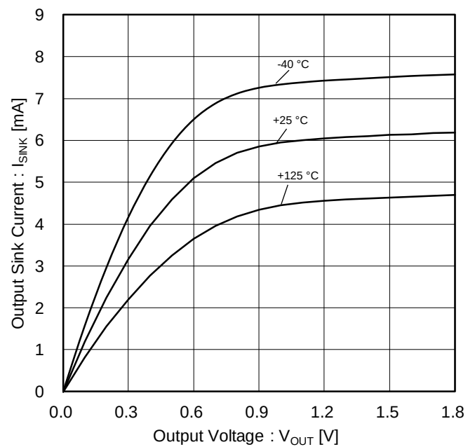
Figure 12. Output Sink Current vs Output Voltage ( V_{DD}=1.8 V)
