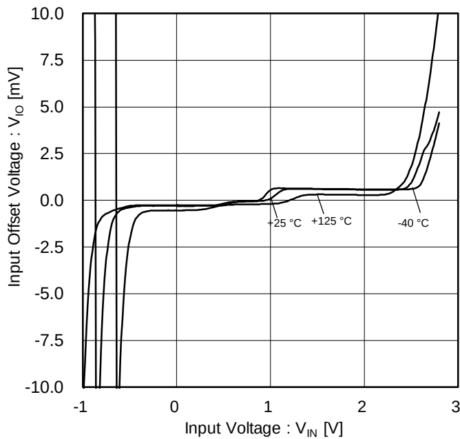
Figure 17. Input Offset Voltage vs Input Voltage ( V_{DD}=1.8\text{ V} )
