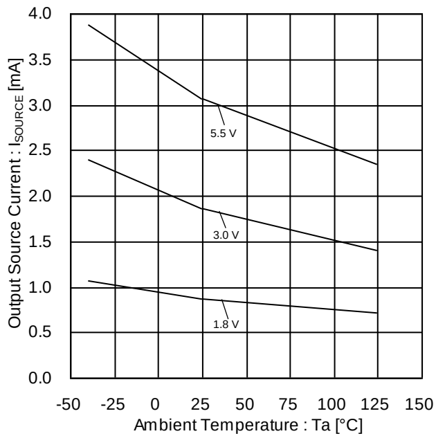
Figure 9. Output Source Current vs Ambient Temperature ( V_{OUT}=V_{DD}-0.4 V)
