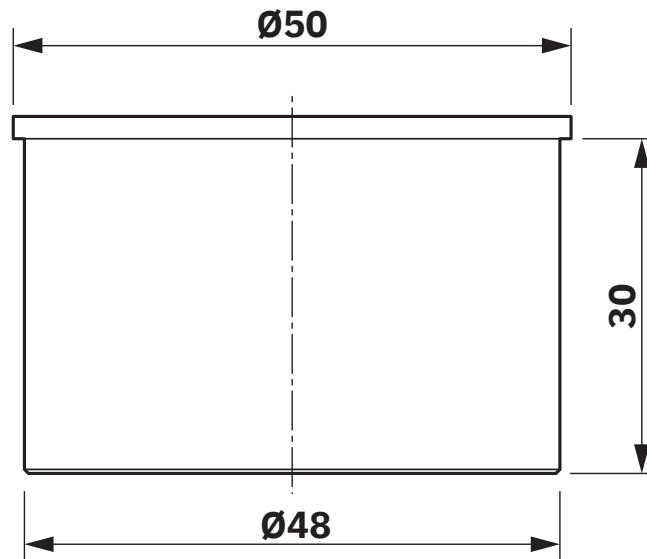
Dimensional drawing
