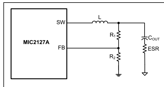
FIGURE 5-4: Enough Ripple at FB.
