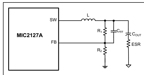
FIGURE 5-5: Inadequate Ripple at FB.
