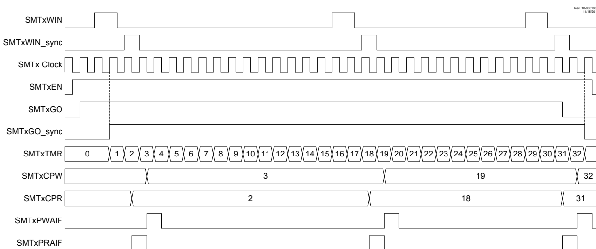
Figure 27-16. Capture Mode, Repeat Acquisition Timing Diagram
