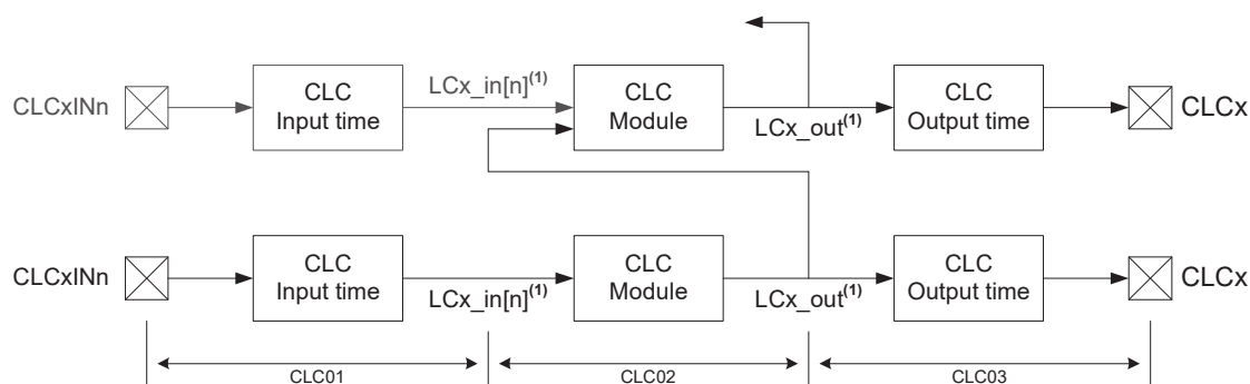
Figure 47-19. CLC Propagation Timing
