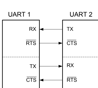
Figure 34-10. Hardware Flow Control Connections
