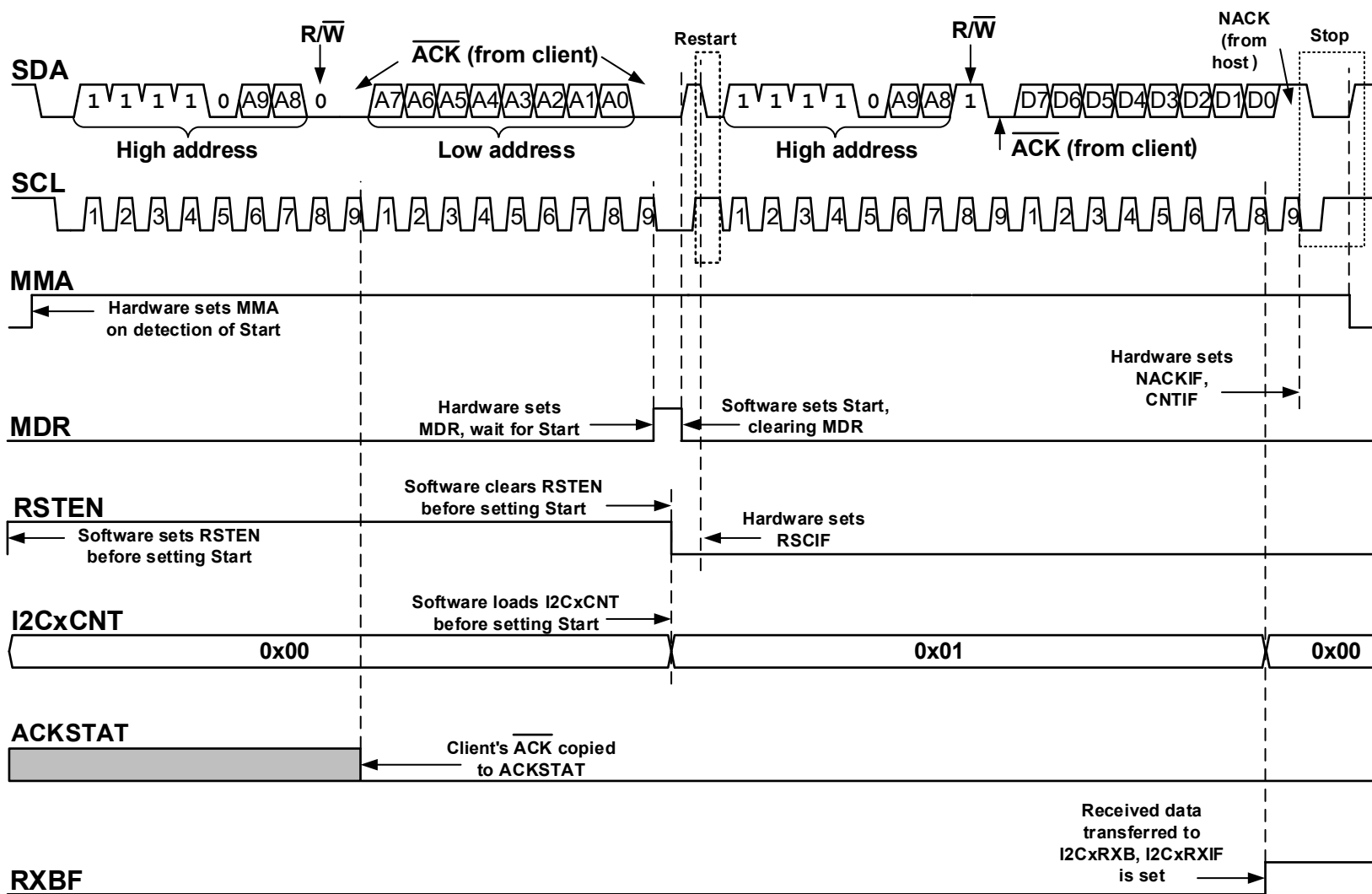
Figure 36-40. 10-Bit Host Mode Reception
