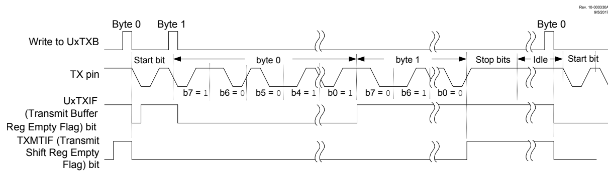
Figure 34-9. Manchester Timing
