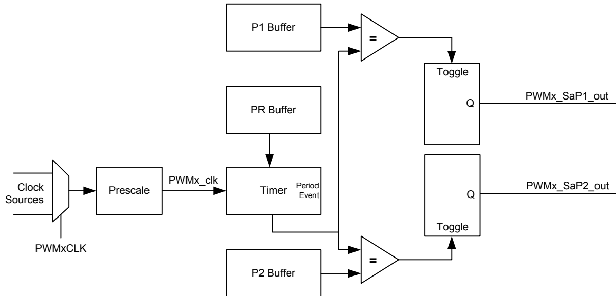
Figure 30-11. Toggled Compare Block Diagram
