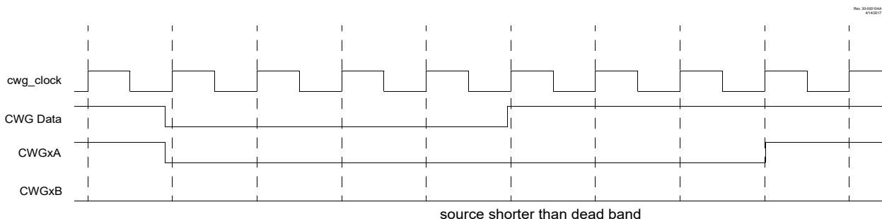
Figure 31-13. Dead-Band Operation, CWGxDBR = 0 \times 03 , CWGxDBF = 0 \times 06 , Source Shorter Than Dead Band
