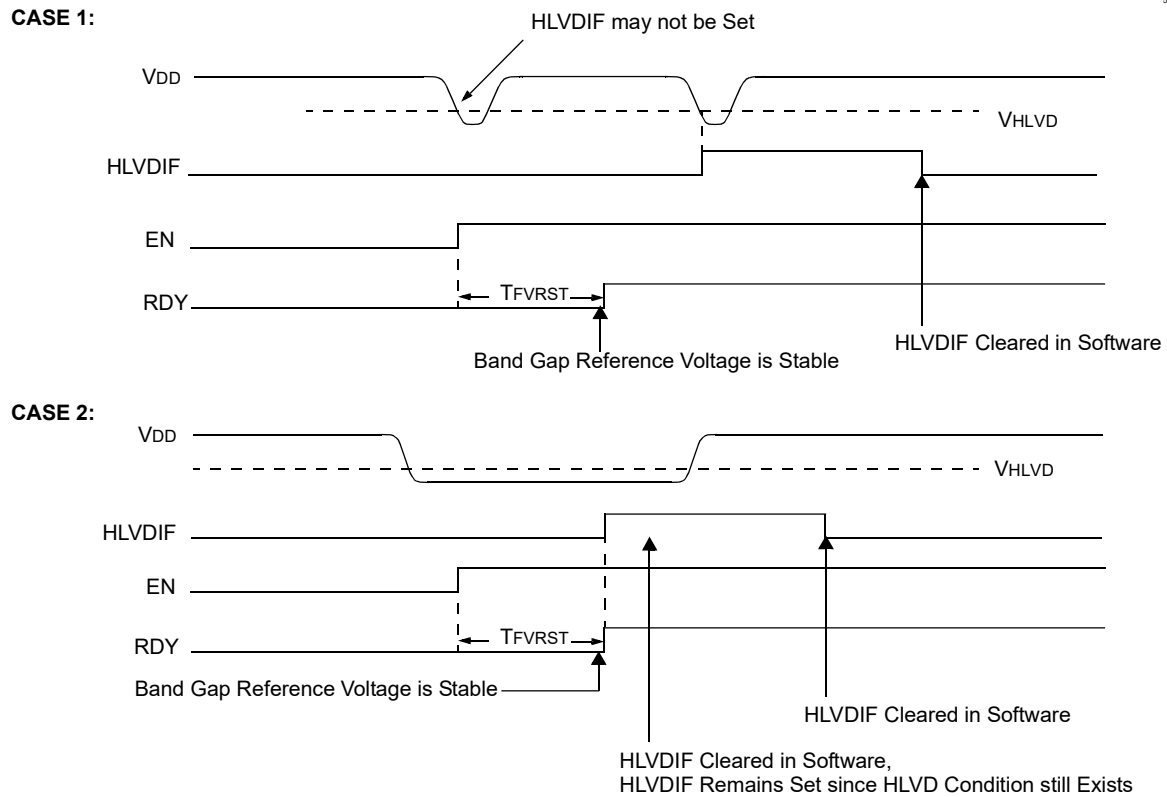
Figure 37-2. Low-Voltage Detect Operation (INTL = 1)
