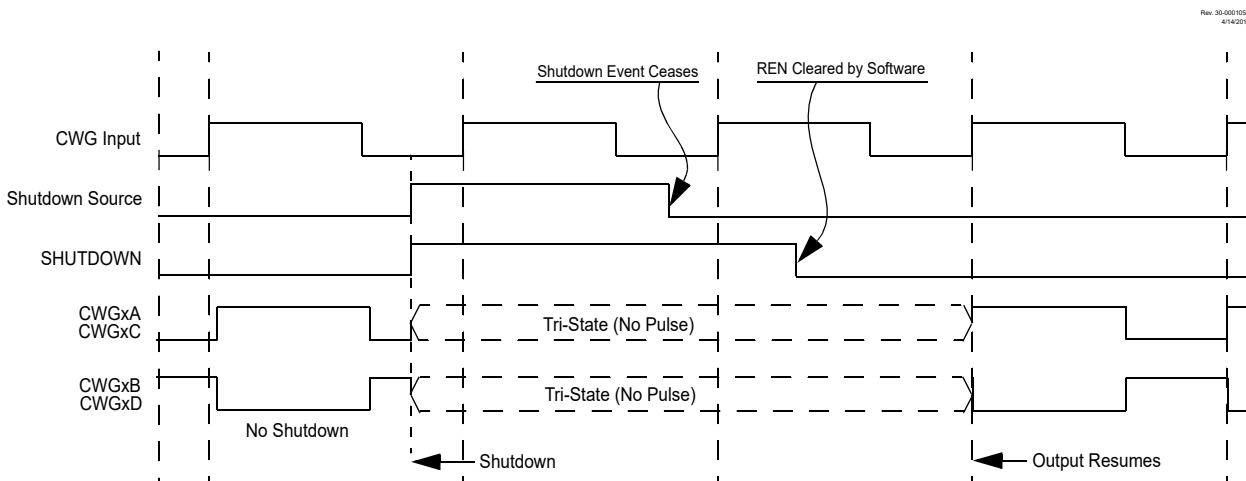
Figure 31-15. Shutdown Functionality, Auto-Restart Disabled (REN = 0, LSAC = 'b01, LSB0 = 'b01)
