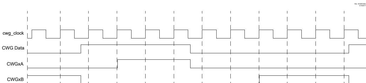
Figure 31-12. Dead-Band Operation, CWGxDBR = 0 \times 01 , CWGxDBF = 0 \times 02
