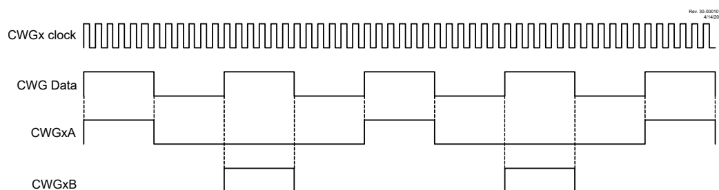
Figure 31-10. Example of Synchronous Steering ( MODE = 'b001)
