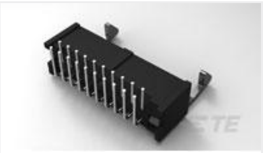
TE Part #2-1761607-6 IDC LOW PRO HDR 16P RA LAT
